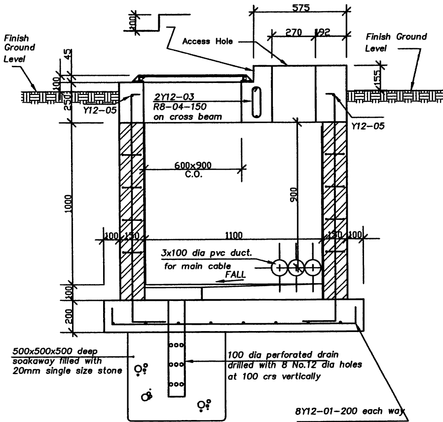
Section Scale 1:20
