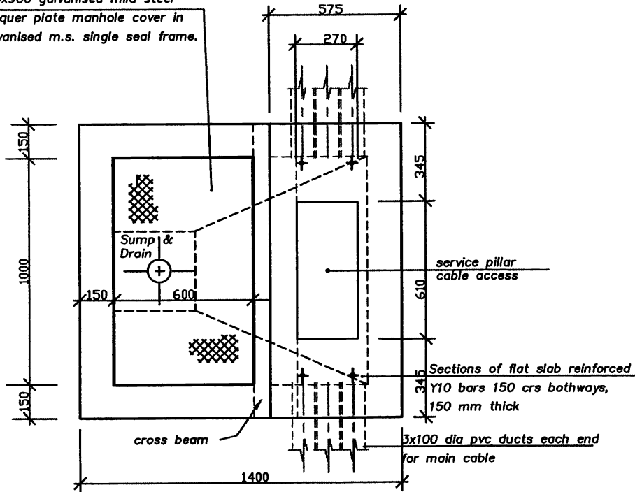
Plan Scale 1:20
