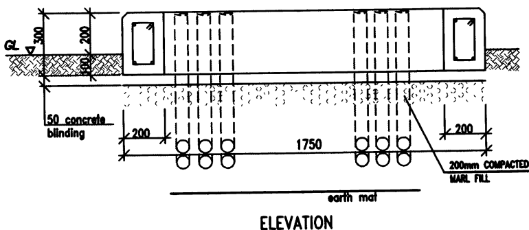
CONCRETE PAD DETAILS THREE PHASE PADMOUNT TRANSFORMER (LOOP FEED)
