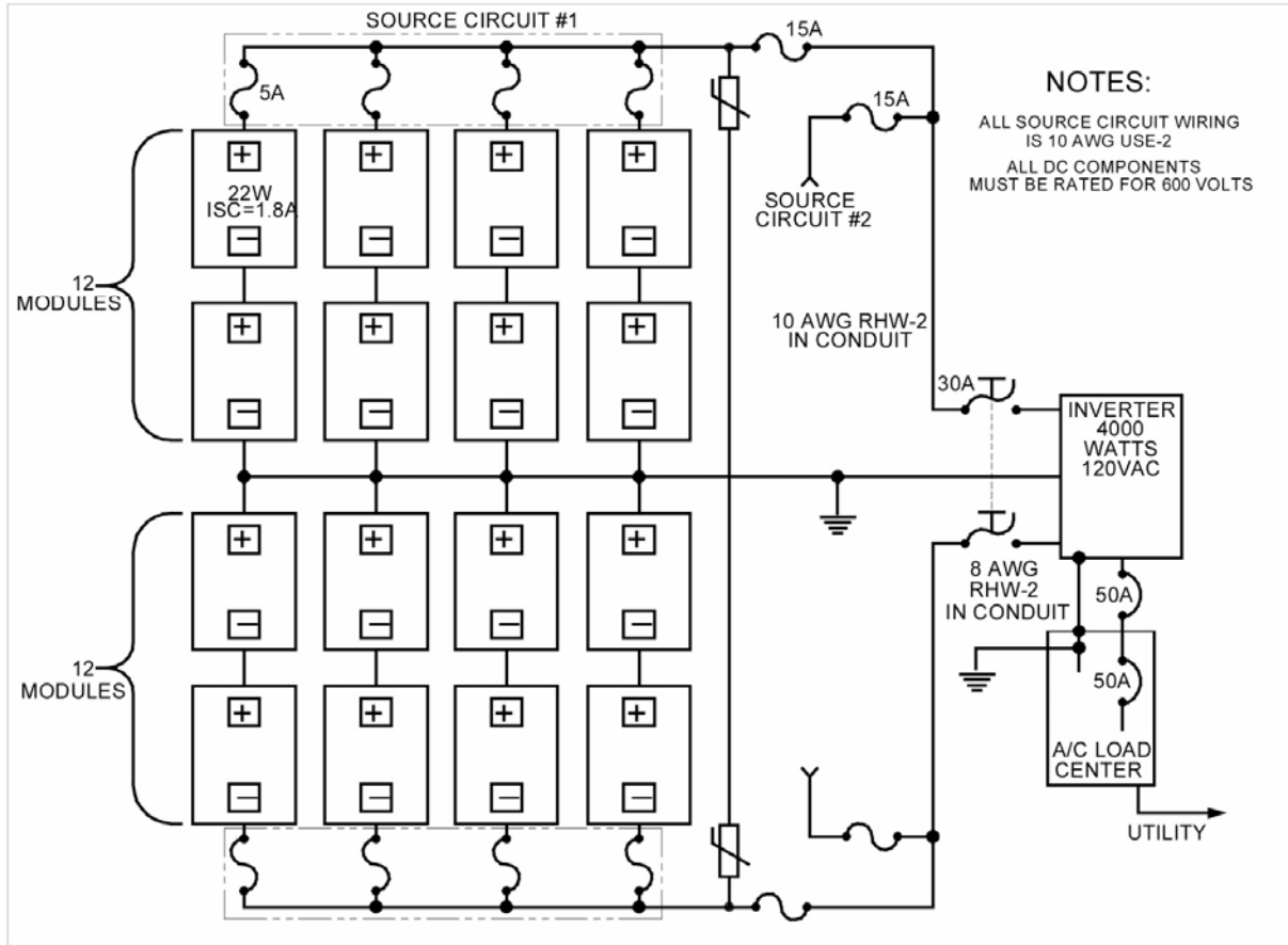
Centre-tapped PV grid-interconnected PV system
