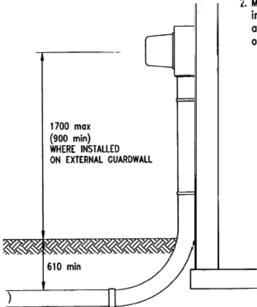
METER SOCKET INSTALLATION UNDERGROUND SERVICE
